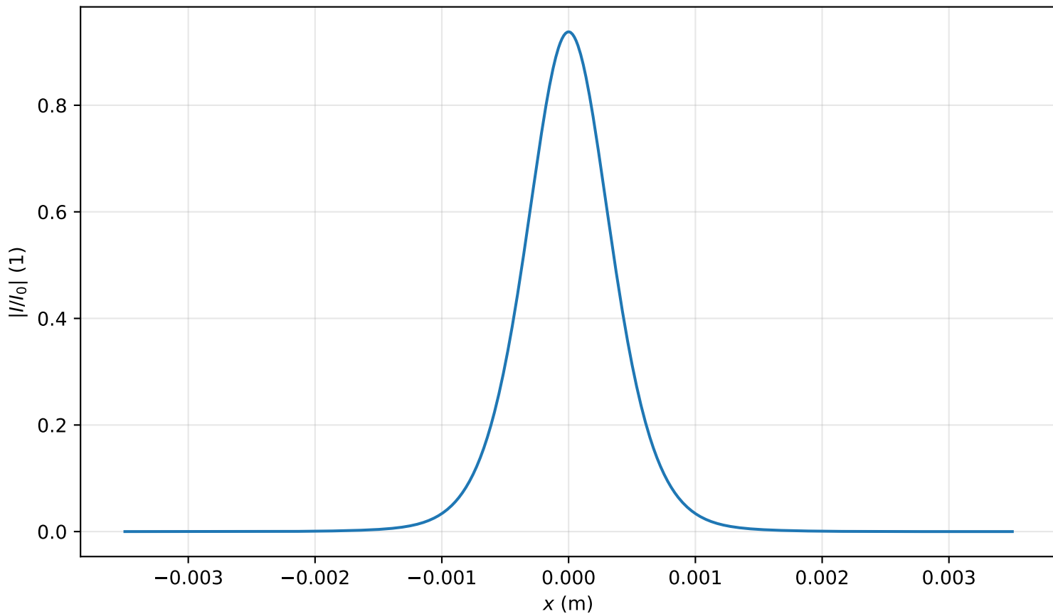
Intensity profile I(x, y = 0, z = 2.627m)/I_0 , P_{in}=0.7P_{cr} , artificial time
